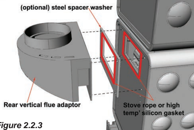
Connection of (optional) Rear Vertical Flue Adaptor
